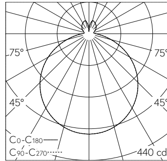
LED 3000 K 13.3 W 1236 lm-h / CIE Flux 45 76 93 86 100 / B43 selon DIN 5040
