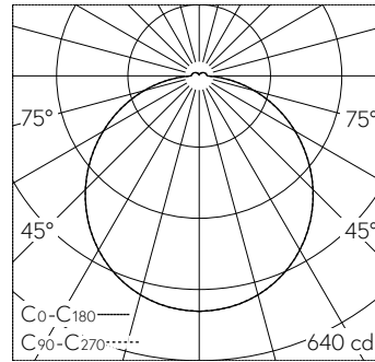
LED 3000 K 22 W 2203 lm-h 116° / CIE Flux 45 75 93 95 100 / A41 selon DIN 5040
