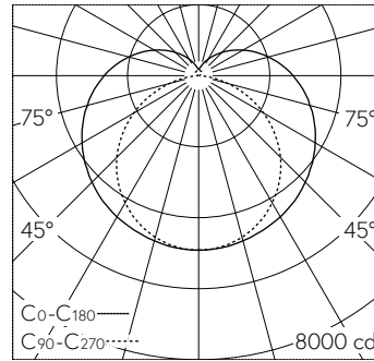
LED 4000 K 218 W 24578 lm-h / CIE Flux 36 64 84 79 100 / B31 selon DIN 5040
