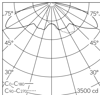
LED 4000 K 67 W 9366 lm-h H = 5 m / CIE Flux 34 68 94 100 100 / A20 selon DIN 5...
