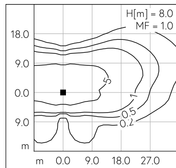
LED 4000 K 67 W 9366 lm-h H = 8 m / CIE Flux 34 68 94 100 100 / A20 selon DIN 5...
