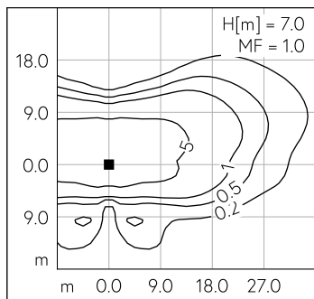
LED 4000 K 67 W 9366 lm-h H = 7 m / CIE Flux 34 68 94 100 100 / A20 selon DIN 5...
