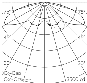
LED 4000 K 67 W 9366 lm-h H = 6 m / CIE Flux 34 68 94 100 100 / A20 selon DIN 5...
