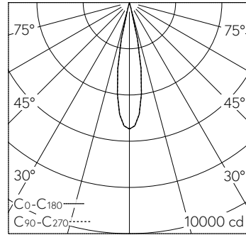
LED 4000 K 43.5 W 585 lm-h 20°_Flood / CIE Flux 100 100 100 100 100 / A80 selon...
