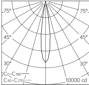
LED 4000 K 43.5 W 585 lm-h 16.0°_Spot / CIE Flux 100 100 100 100 100 / A80 selon...
