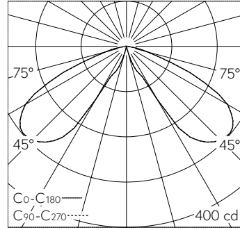
LED 4000 K 3,0 W 418 lm-h 132° / CIE Flux 24 73 97 99 100 / A20 selon DIN 5040
