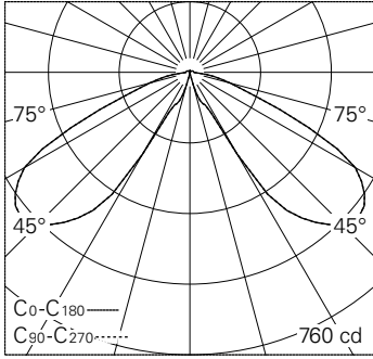
LED 4000 K 19.5 W 1933 lm-h 132° / CIE Flux 22 72 96 98 100 / A21 selon DIN 5040
