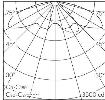
LED 3000 K 33.5 W 4554 lm-h H = 8 m / CIE Flux 34 68 94 100 100 / A20 nach DIN ...
