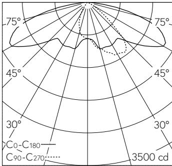
LED 3000 K 33.5 W 4554 lm-h H = 7 m / CIE Flux 34 68 94 100 100 / A20 nach DIN ...
