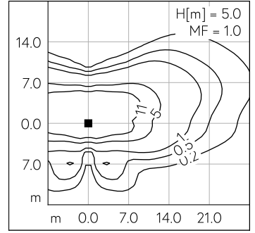
LED 3000 K 33.5 W 4554 lm-h H = 5 m / CIE Flux 34 68 94 100 100 / A20 nach DIN ...
