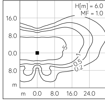
LED 3000 K 33.5 W 4554 lm-h H = 6 m / CIE Flux 34 68 94 100 100 / A20 nach DIN ...
