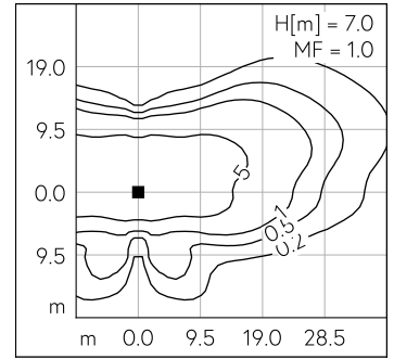
LED 3000 K 51.2 W 6904 lm-h H = 7 m / CIE Flux 34 67 93 100 100 / A20 nach DIN ...
