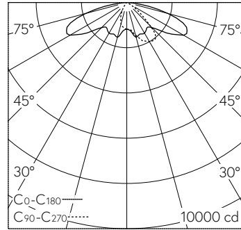
LED 3000 K 51.2 W 6904 lm-h H = 7 m / CIE Flux 34 67 93 100 100 / A20 nach DIN ...
