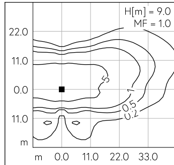
LED 3000 K 51.2 W 6904 lm-h H = 9 m / CIE Flux 34 67 93 100 100 / A20 nach DIN ...
