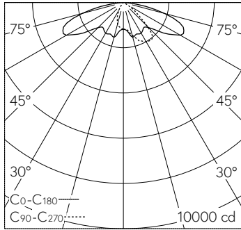
LED 3000 K 51.2 W 6904 lm-h H = 8 m / CIE Flux 34 67 93 100 100 / A20 nach DIN ...
